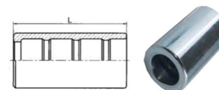
Ferrule for R7/R8 - 00018
