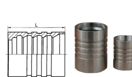
Non-Skive Ferrule for 4SH;R12/32 00401
