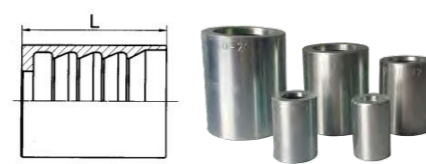
Non-Skive ferrule for 2SN/R2AT-00210
