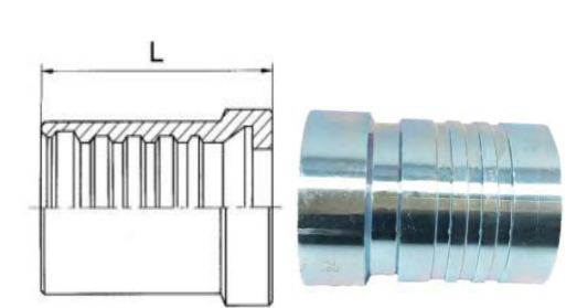
Skive inner & outer rubber Ferrule for 4SH -000421
